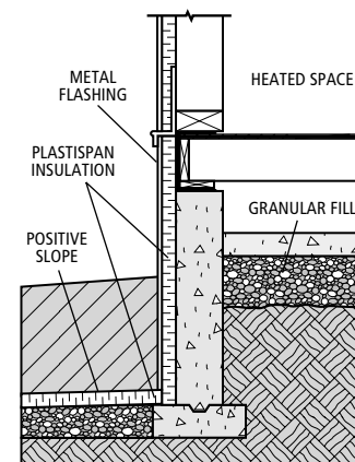
Figure 2. Insulation Detail for Heated Structures
