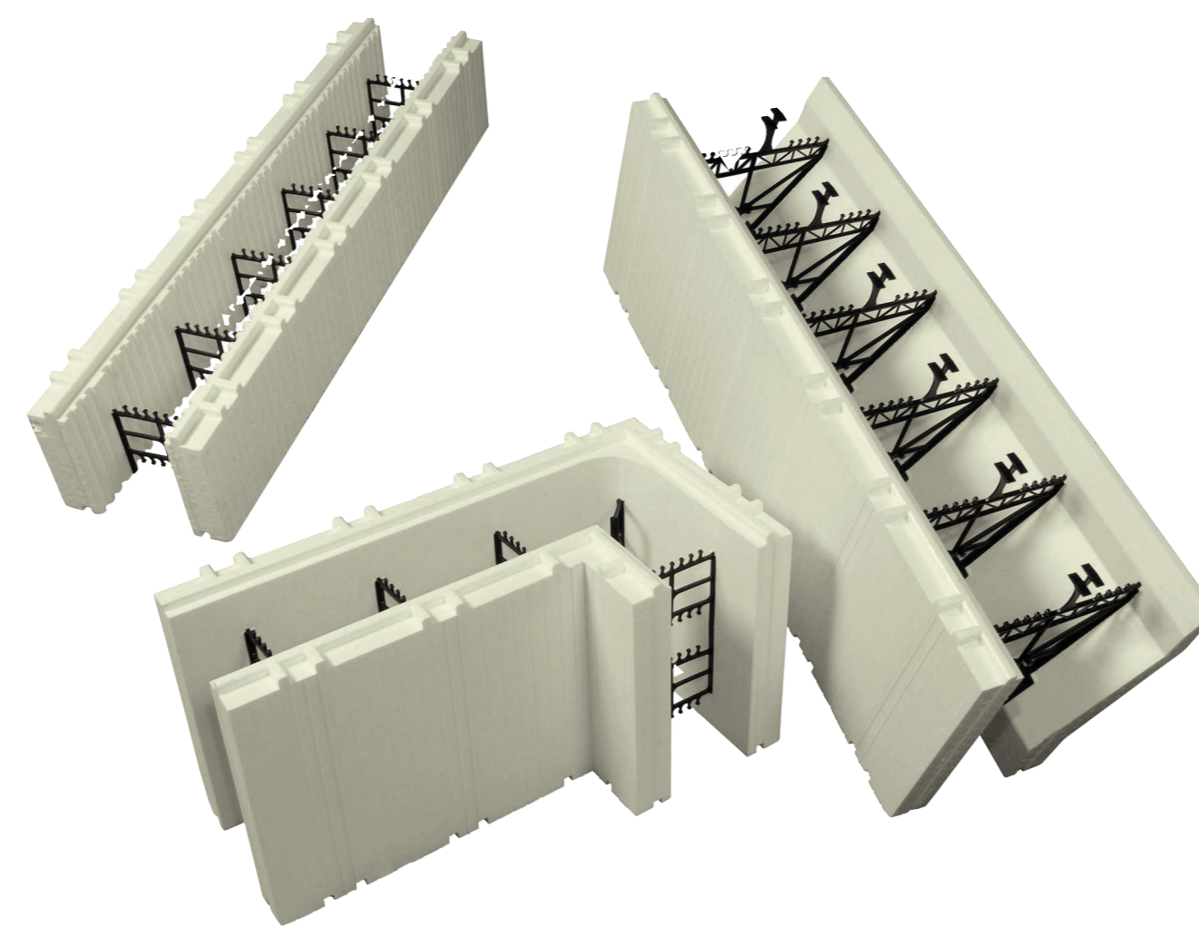
Advantage ICF System® Insulating Concrete Forming System
