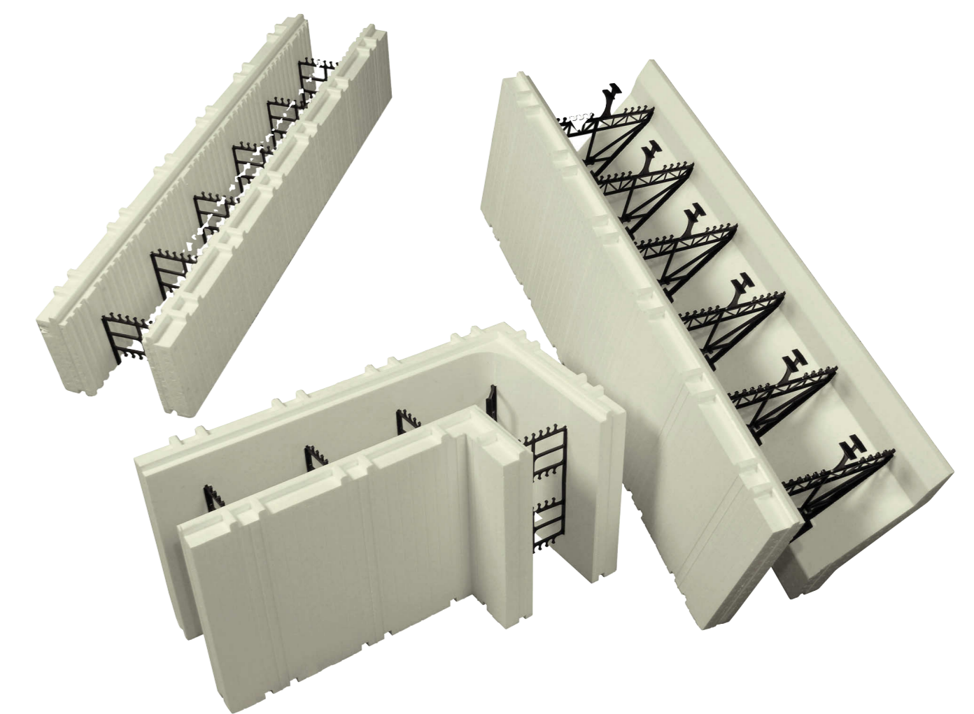
Advantage ICF System® Insulating Concrete Forming System
