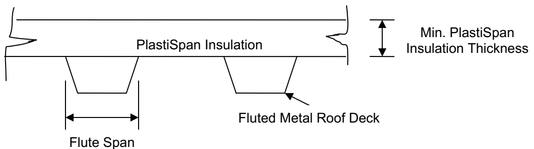
Figure 2 - PlastiSpan Insulation Minimum Thickness
